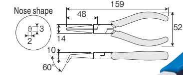
P-12 MINIATURE ROUND NOSE PLIERS 弯嘴尖头钳
