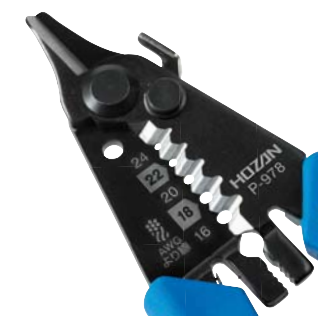
P-978 For medium-to-thick wires 中太線用
