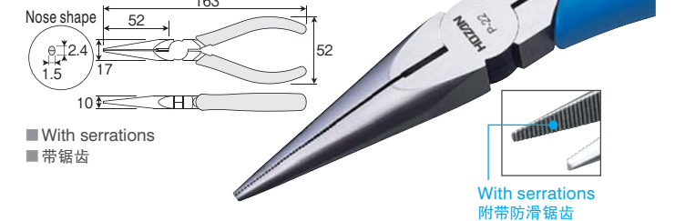
P-22 LONG NOSE PLIERS WITH SIDE CUTTER 尖头钳
