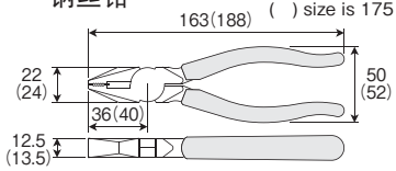
P-43-150/175 LINEMAN'S PLIERS 钢丝钳
