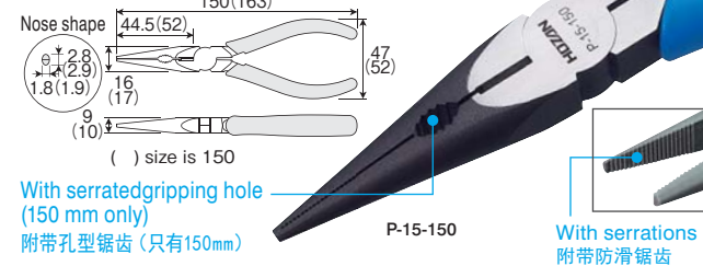
P-15-125/150 LONG NOSE PLIERS WITH SIDE CUTTER 尖头钳
