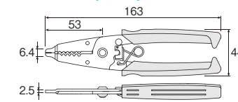
P-968 For medium-to-thick wires 中太線用
