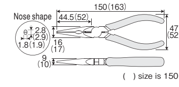
P-22 LONG NOSE PLIERS WITH SIDE CUTTER 尖头钳
